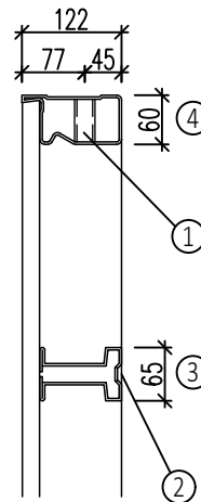
Profiles
