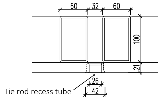
Section of integral bracing showing tie rod hole
