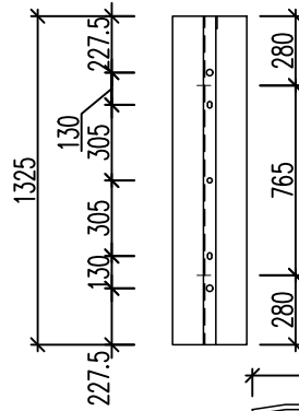
1325 mm high
