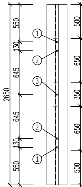
2650 mm high
