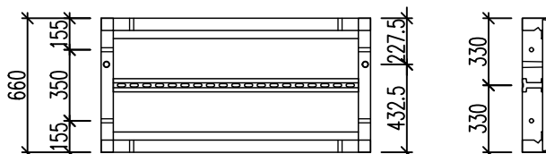
Section
