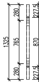
1325 mm high
