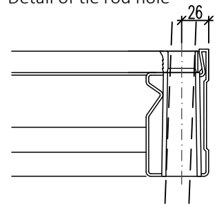
Detail of tie rod hole
