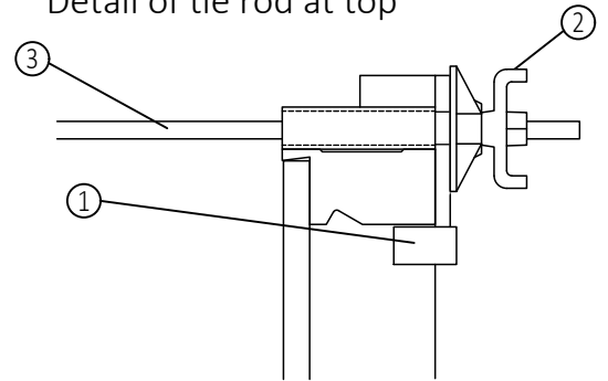
Detail of tie rod at top
