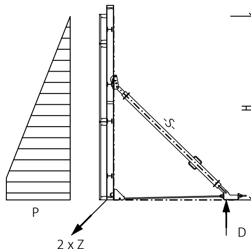
Version II: NOEtop bracing
