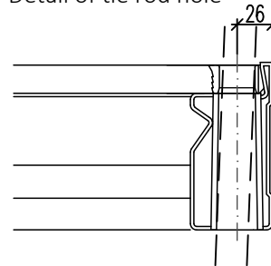
Detail of tie rod hole
