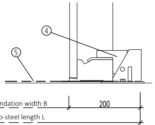
Detail with tie at bottom Tie with foundation clamp
