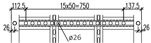
Dimensions of holes through channel
