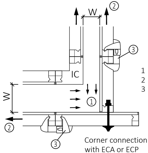
External corner
