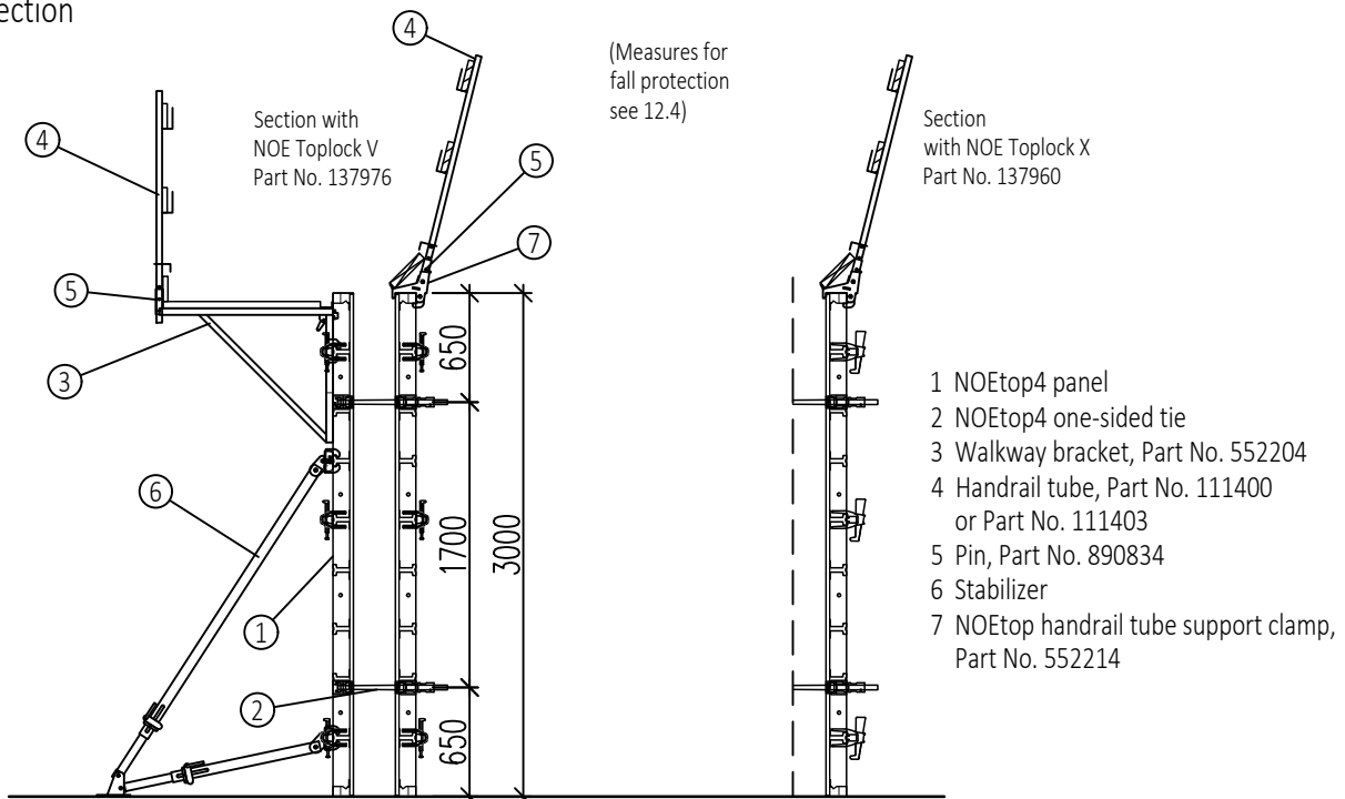
Butt joint with Toplock V Part No. 137976
