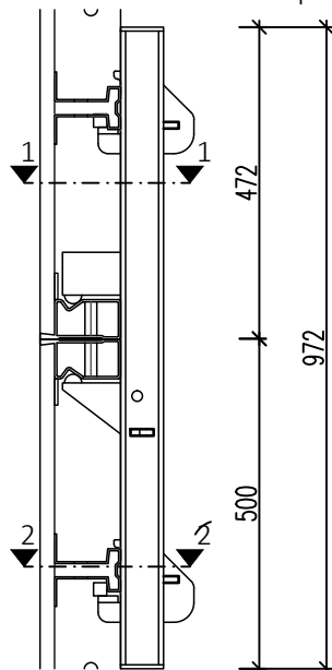
Extension with end-on panels
