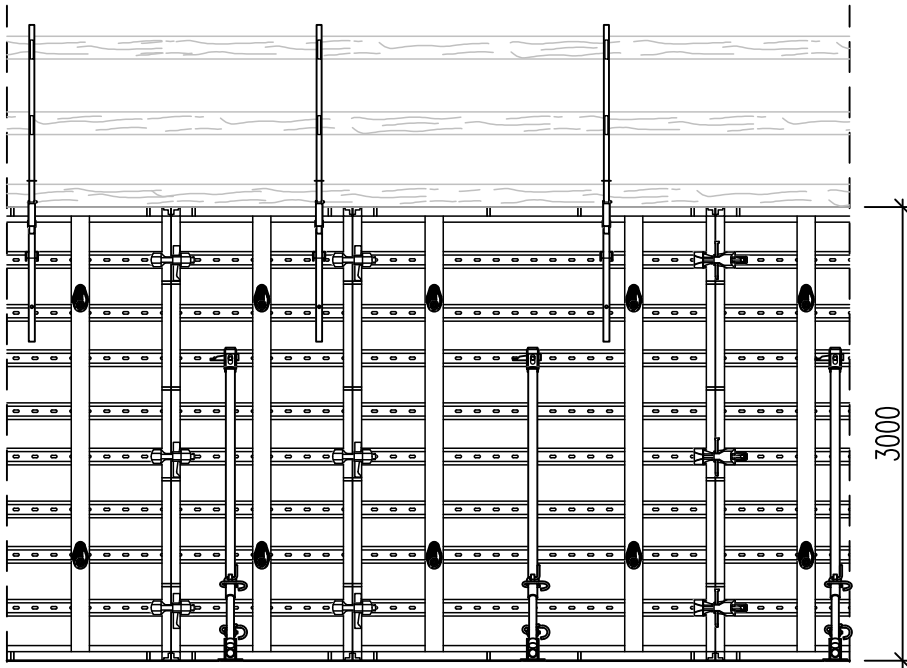
Butt joint with Toplock V Part No. 137976
