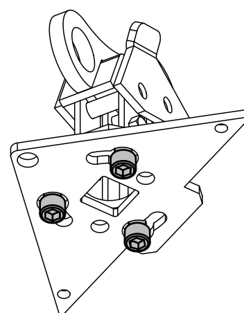
View from below: Cover plate and lever head with bayonet lock ("bayonet lock")
