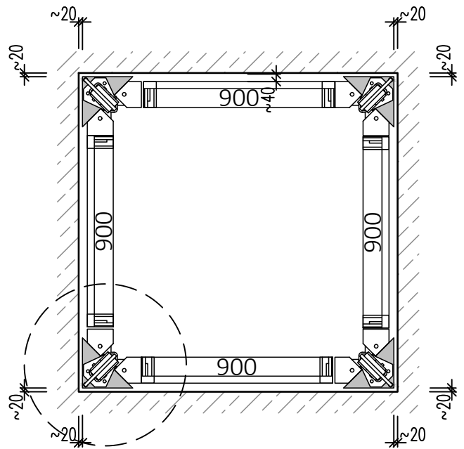
Example of formwork in stripping setting
