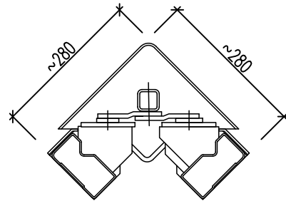
◆ Cross-section Stripping corner in stripping setting
